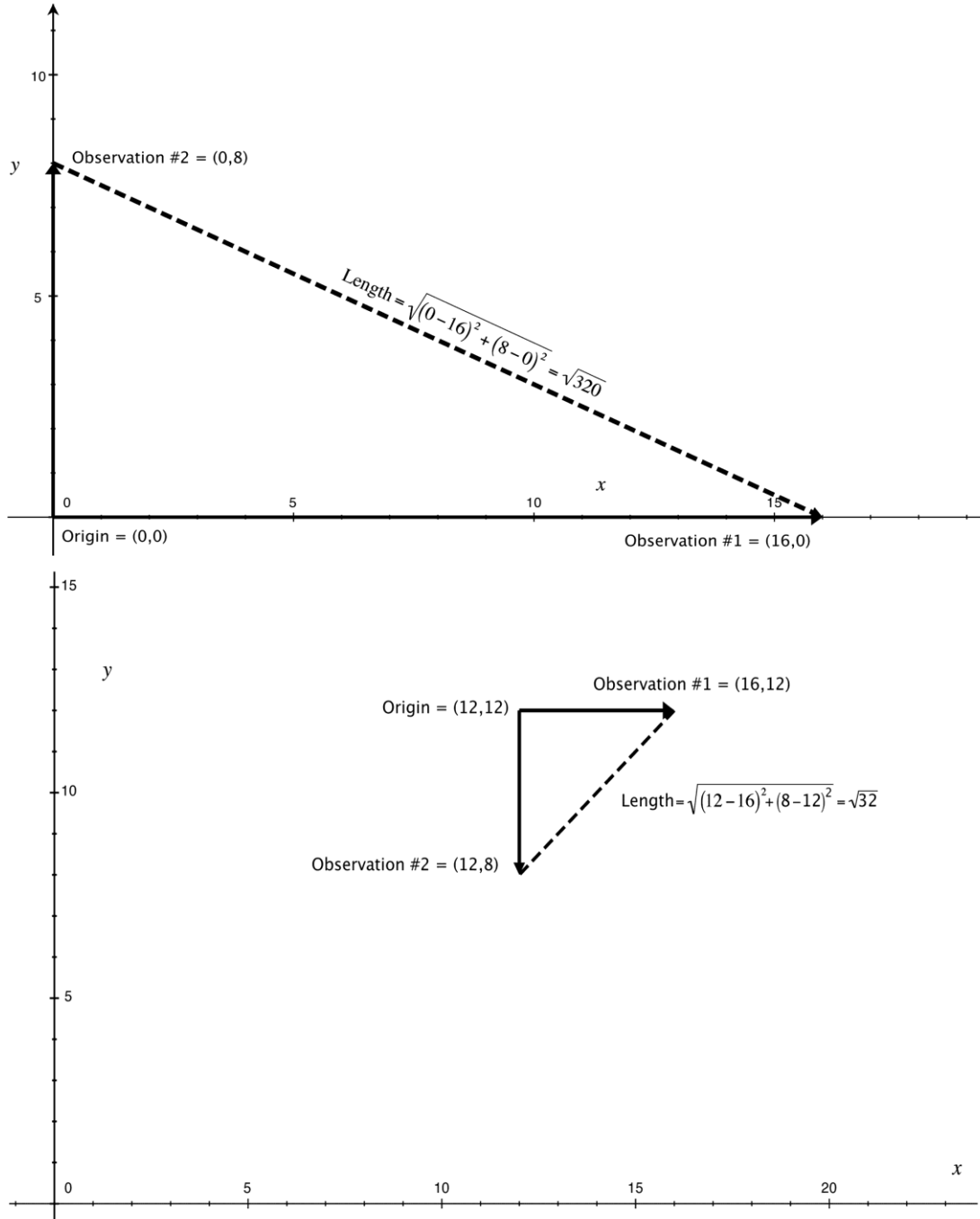
Figure 3. A geometric representation of the least squares criterion. A distribution of two independent observations \{8,16\} can be represented as orthogonal vectors. Joining the two vectors produces a right triangle. The length of the hypotenuse of the triangle is the square root of the sum of squared deviations of the observations from the origin. The top graph demonstrates the length of the hypotenuse (dashed line) when the origin is set at (0,0) . The bottom graph demonstrates the length of the hypotenuse (dashed line) when the origin is set at the value of the mean (12,12) . If the mean is used as the origin, the length of the hypotenuse (i.e. sum of squared deviations) is at a minimum.
