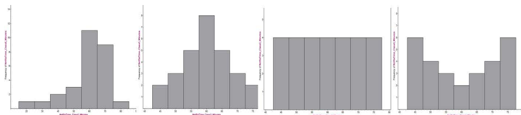
Figure 1: Histograms of the four distributions (skewed, normal, uniform, & inverted bell curve).
