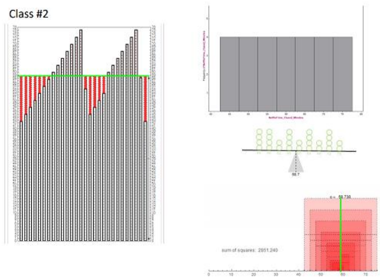
Figure 2: Second ranking task with the different interpretations from the Mathematica tool (leveling off, histogram, balance beam, and the sum of squares).
