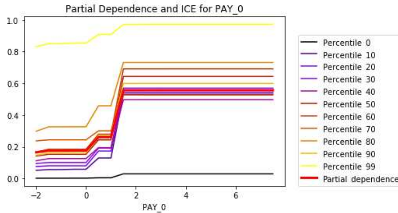
Figure 8: Partial dependence and ICE curves for learned GBM response function g_{\text{mono}} and important input feature PAY_0 in a 30% validation set randomly sampled from the UCI credit card dataset.
