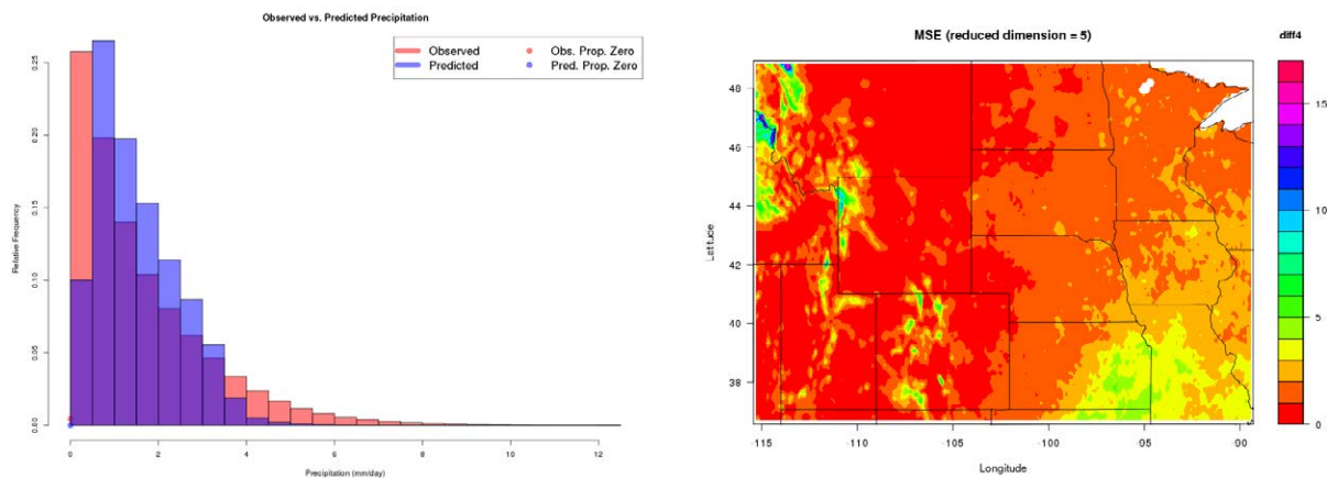
(a) Observed and predicted monthly precipitation, including the proportion of 0 values for both (b) MSE from positive predictions for months with positive rainfall (true positives)
