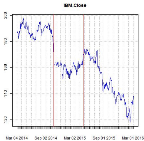
Figure 1: Estimated Changepoints in IBM Prices.
