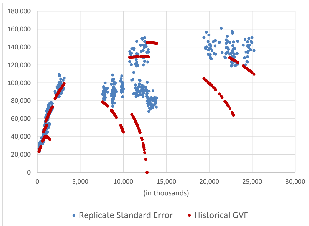
Figure 2: Replicate and GVF standard errors (vertical axis) plotted against associated survey estimates of employed, unemployed, and not in labor force for Hispanic, 20 and older and Hispanic, 16 and older .
