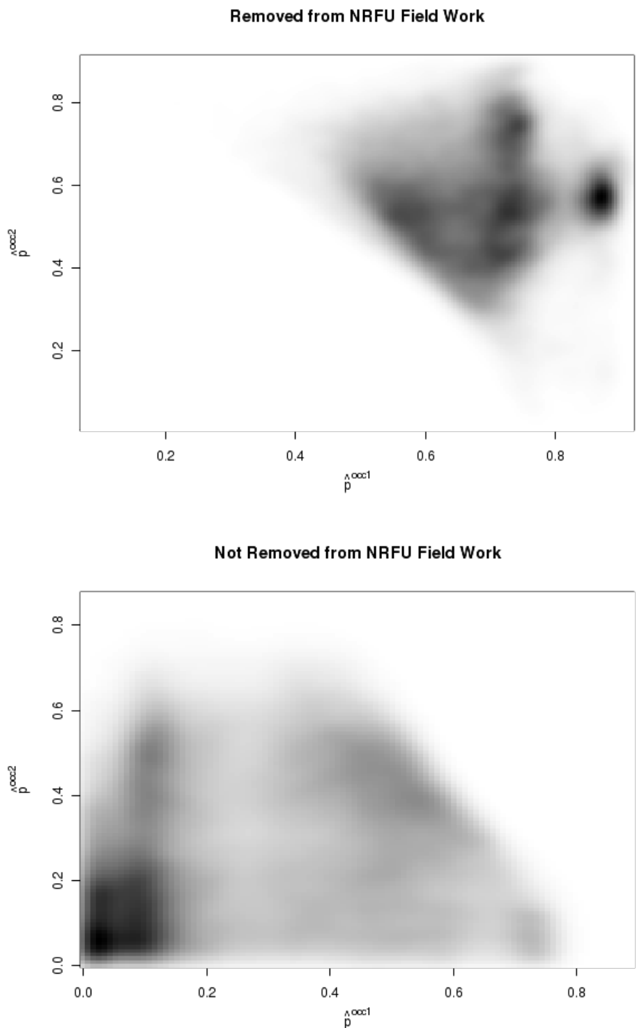
Figure 3: Bivariate Distributions of Housing Unit Predicted Probabilities by Administrative Record Usage for Occupied Models in Selected Scenario: Darker shading is higher density.
