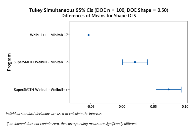
Figure 9: Tukey means plot of LS \beta for DOE n = 100, DOE Shape = 0.50
