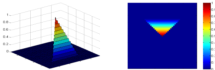
Figure 5: Example of a facet-like linear function over two-dimensional Euclidean space.
