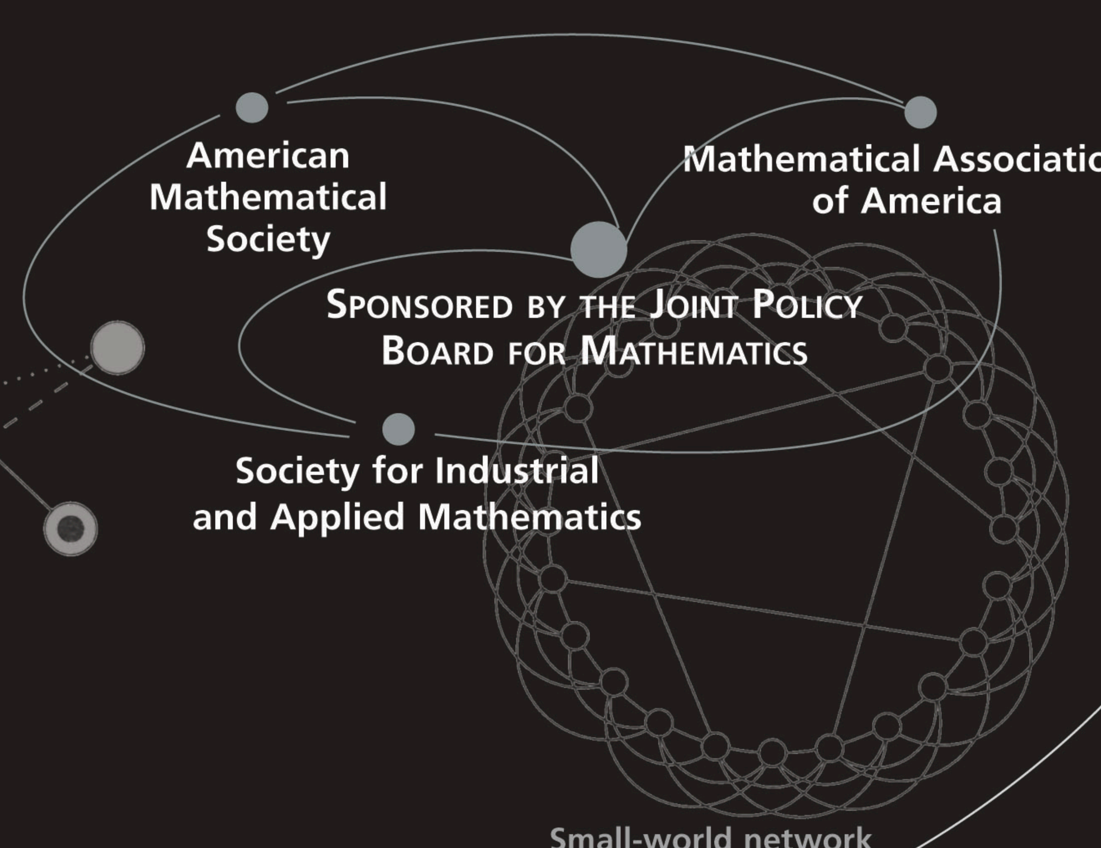
Small-world network
