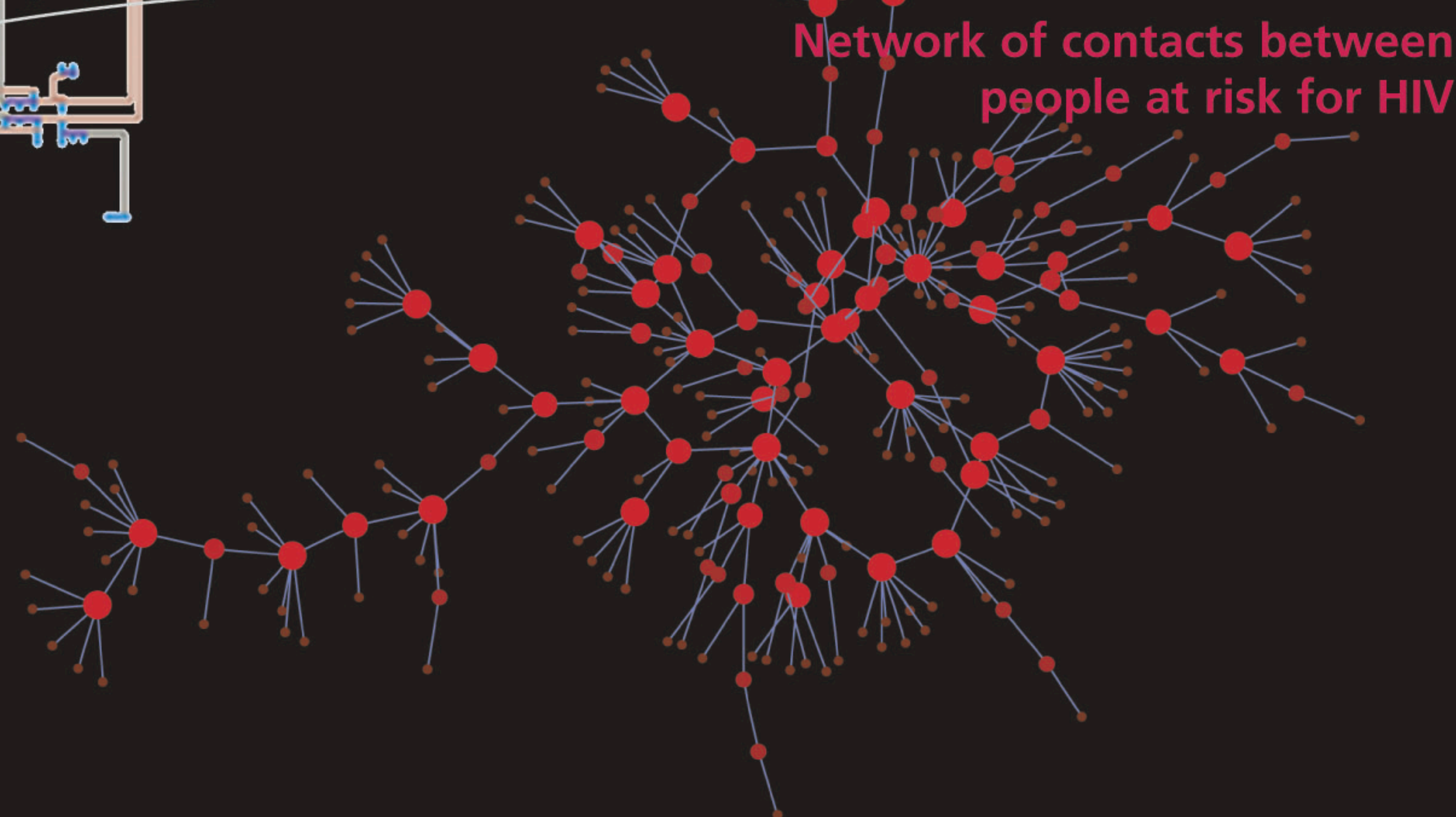
Scale-free network
