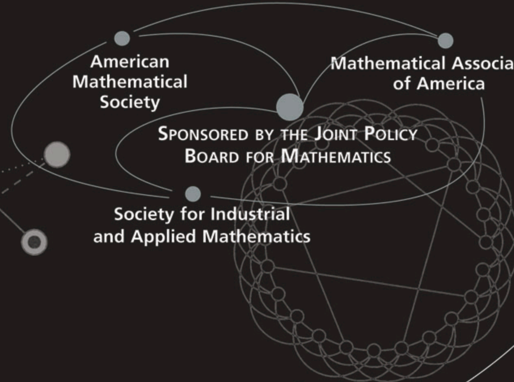
Small-world network
