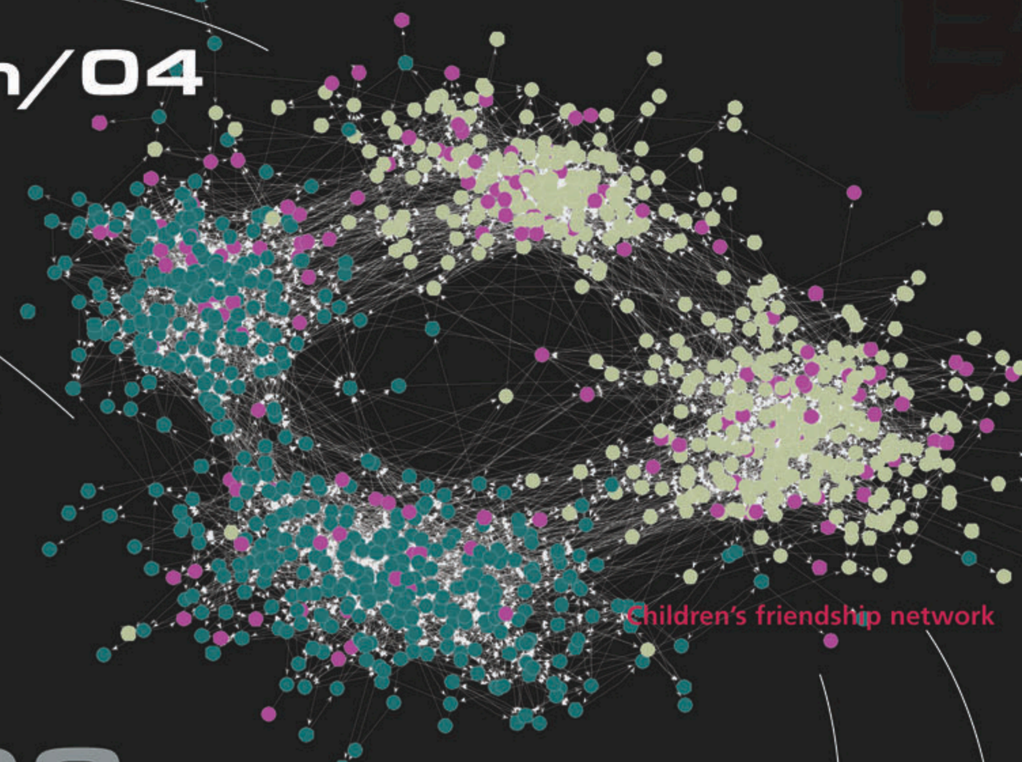
Site percolation in a network
